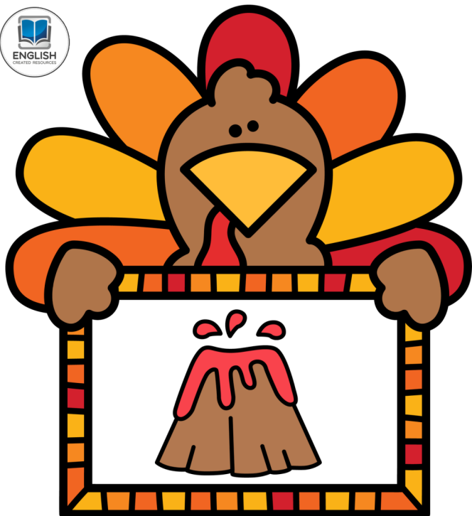
volcano
